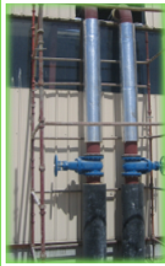
Pumps with Pressure Set-up
